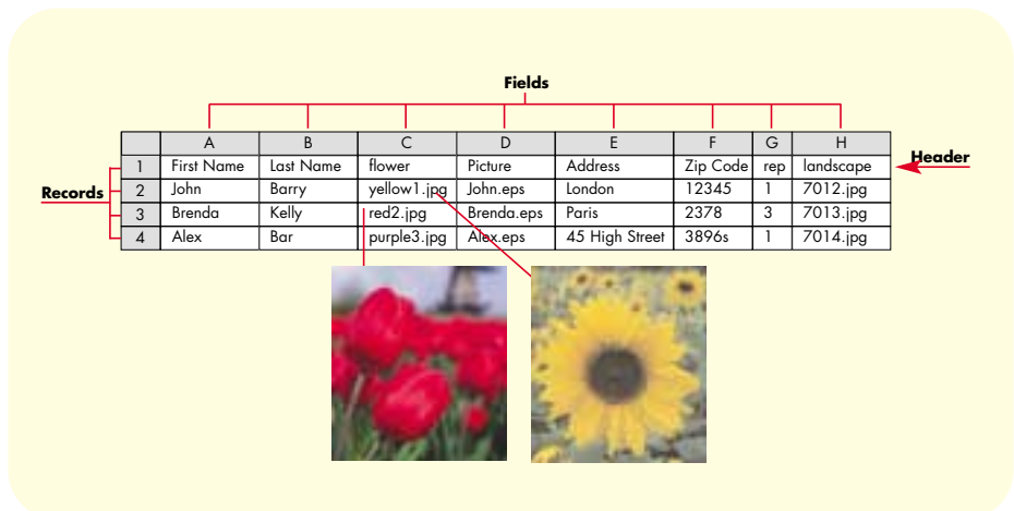
Figure 2. Database structure
